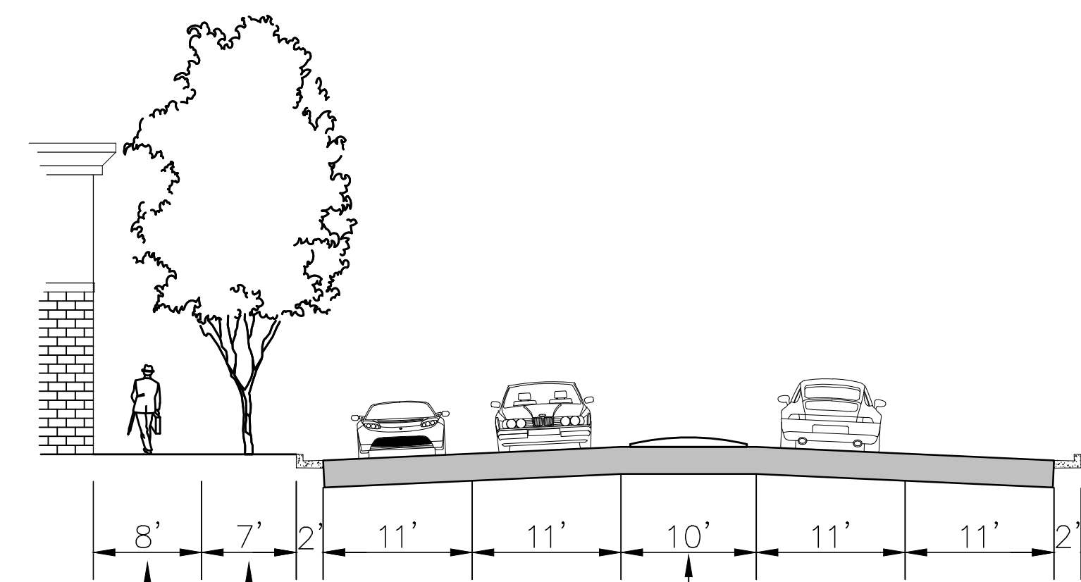
8' PEDESTRIAN ZONE 7' TREE ZONE PIEDMONT ROAD SECTION VIEW: PIEDMONT ROAD N.T.S.
